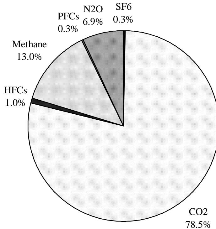
Figure 1.1 EU Global Warming Emissions, 1995 Mtonnes CO 2 equiv.
